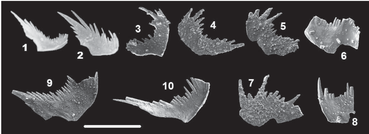
Text-fig. 10. Form-species of Kamuellerella (Neobelodina) brevibasalis Gedik and some new Kamuellerellids . 1-4 – K. (Neobelodina) brevibasalis ; 5-10 – New forms; 1-2 specimens of Gedik (1975); all others from Kılıç (2004), Anisian. Scale bar 100 \mu m
