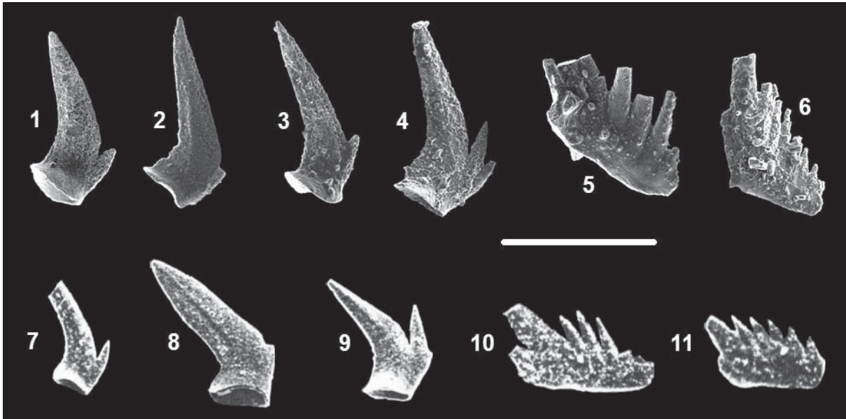
Text-fig. 1. Tethyan cornudinid elements: 1-4, 7-9 – Cornudina oezdemirae Gedik, 1975; 5-6, 10-11 – Cornudina ? latidentata Kozur and Mostler, 1970. 7-11 – specimens of Gedik (1975) and others from Kılıç (2004). Scale bar 150 \mu m
