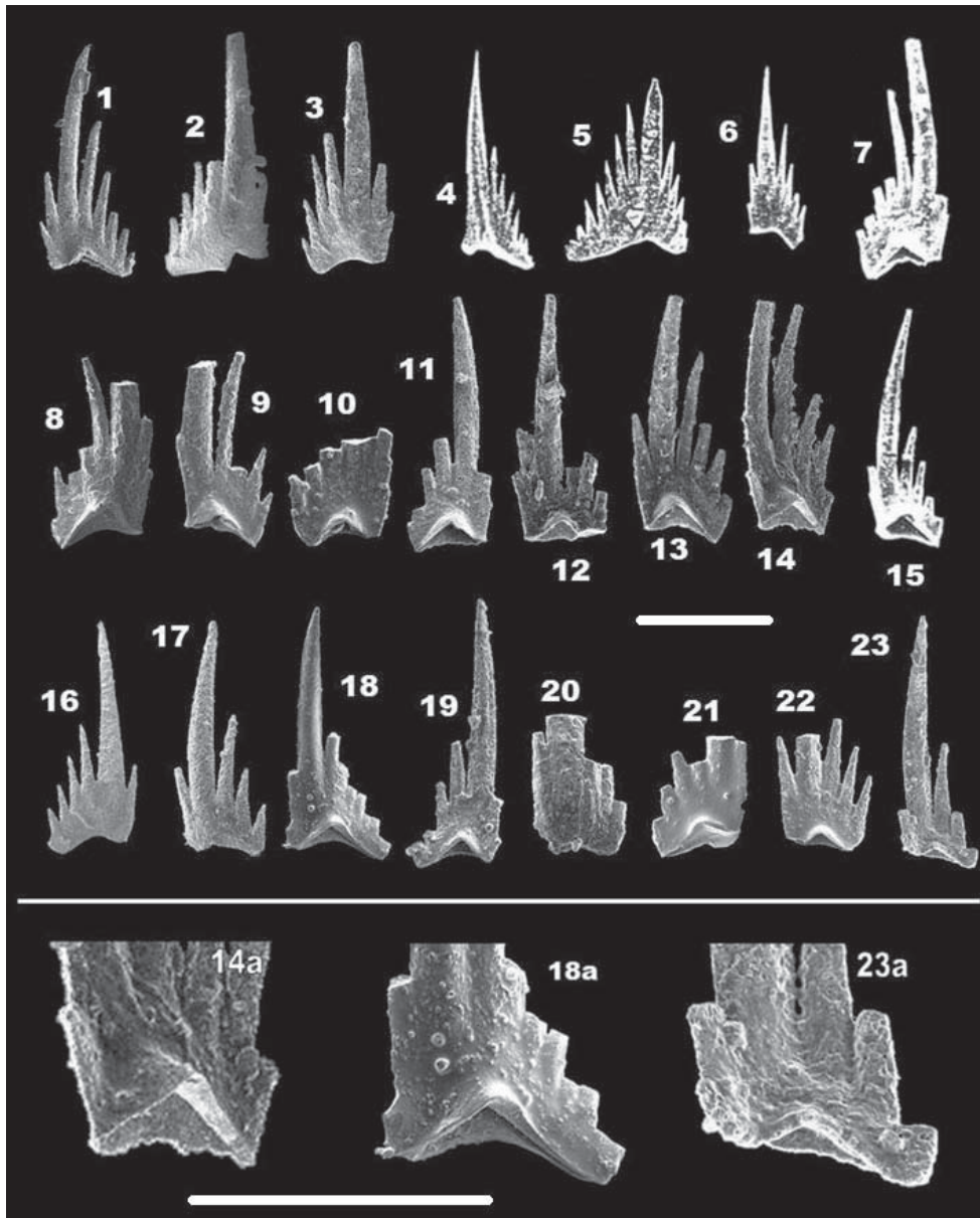
Text-fig. 4. Form-species of Ketinella Gedik, 1975. 1-5 – K. langeri Gedik, 1975; 6-15 – K. maxicavata Gedik, 1975; 16-23 – K. goermueshi sp. nov.; 18, 18a – holotype, 4-7, and 15 are from Gedik (1975), others from Kılıç (2004); Anisian. Scale bar 75 \mu m
