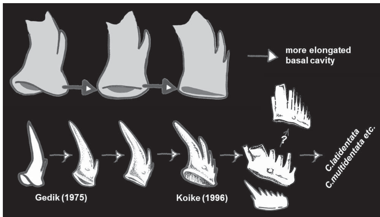
Text-fig. 5. The growth of the basal cavity is proportionately to the progress of the anterior process in Cornudina
