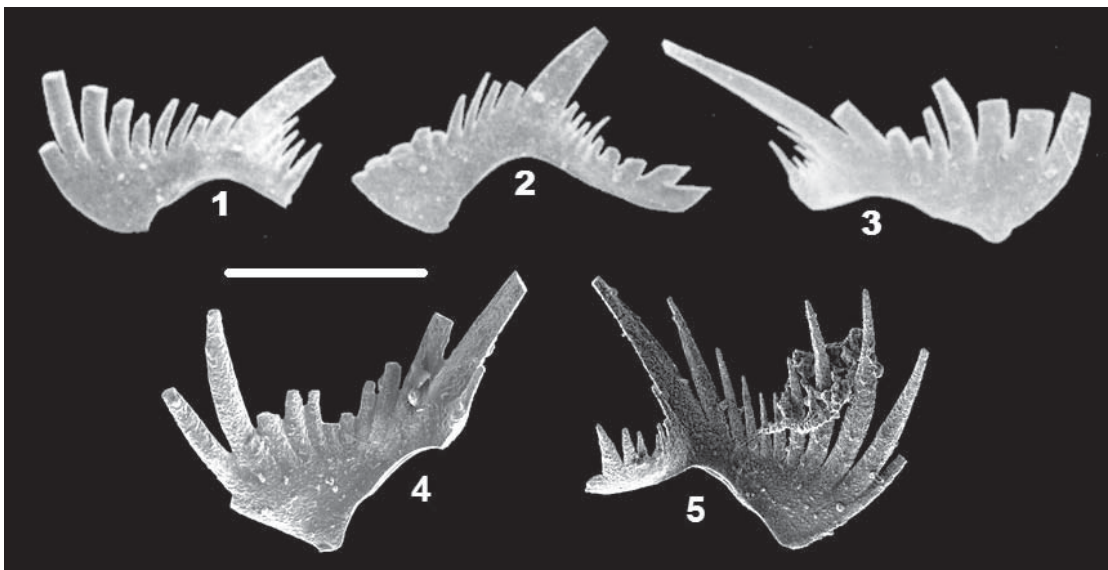
Text-fig. 8. Form-species of Kamuellerella gebzeensis Gedik, 1975. 1-3 – specimens of Gedik (1975); 4-5 – from Kılıç (2004); Anisian. Scale bar: 150 \mu m
