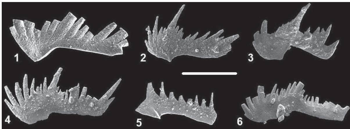
Text-fig. 6. Some ramiform elements (Kılıç 2004) proposed for multielement Cornudina Hirschmann, 1959. 1 – Hindeodella suevica (Tatge, 1956); 2-3 – Neohindeodella triassica (Müller, 1956); 4 – N. Aequiramosa Kozur and Mostler, 1970; 5 – N. Dropla Spasov and Ganev, 1960; 6 – Veghella delicatula Budurov, 1960. Scale bar: 150 \mu m
