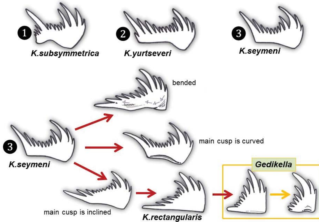
Text-fig. 9. Evolutional relationship between the Kamuellerellids ( Kamuellerella subsymmetrica Gedik, 1975, K. yurtseveri Gedik, 1975, K. seymeni Gedik, 1975, K. rectangularis sp. nov.) and Gedikella quadrata gen.nov. sp. nov.
