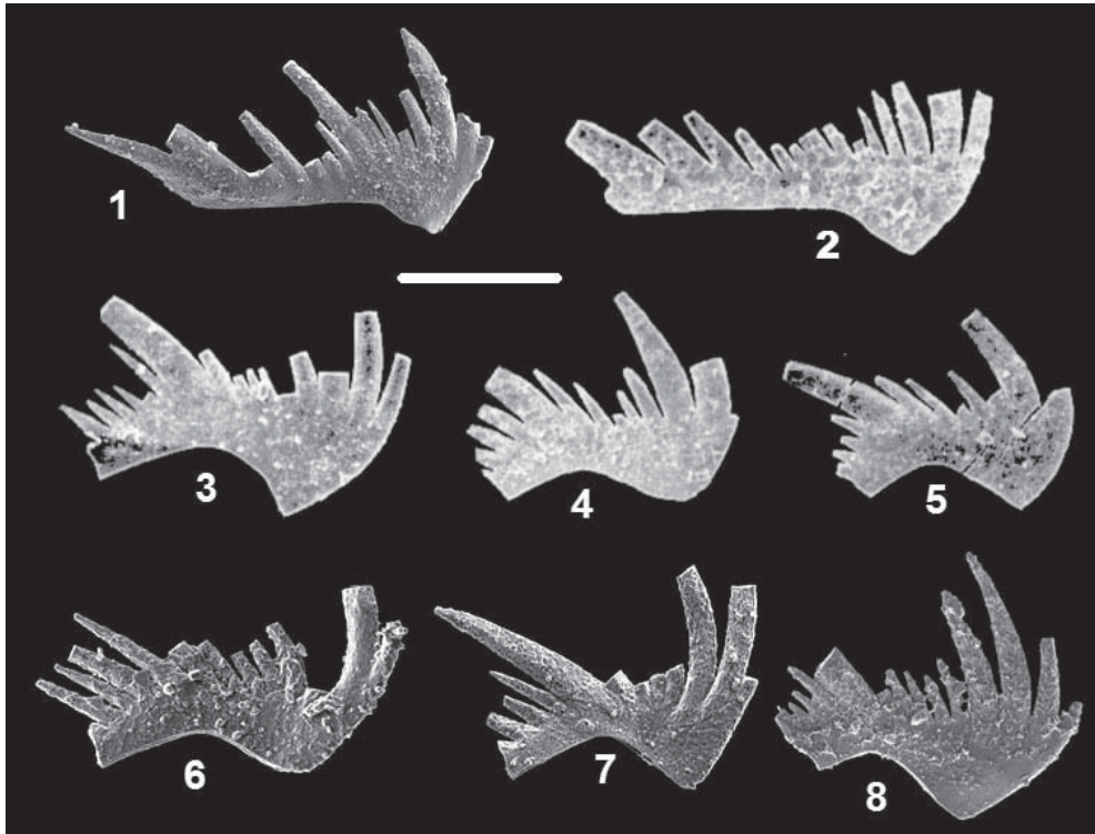
Text-fig. 7. Form-species of Kamuellerella subsymmetrica Gedik, 1975 and K. yurtseveri Gedik, 1975. 1-2 – K. subsymmetrica Gedik, 1975; 3-8 – are K. yurtseveri Gedik, 1975. 2-5 are specimens of Gedik (1975), others from Kılıç (2004); Anisian. Scale bar 150 \mu m
