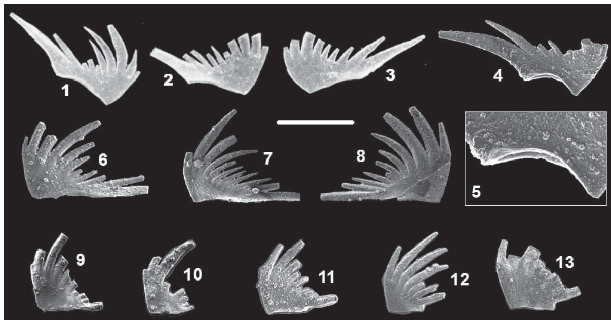
Text-fig. 3. Form-species of Kamuellerella seymeni Gedik, 1975, Kamuellerella rectangularis sp. nov. and Gedikella quadrata gen. nov. sp. nov.; 1-6 – Kamuellerella seymeni Gedik, 1975; 6 – bended form; 7 – transitional form between K. seymeni and K. rectangularis sp. nov.; 8 – Kamuellerella rectangularis sp. nov.; 9-13 – Gedikella quadrata gen. nov. sp. nov.; 9 – holotype, 10-13 – paratypes. Anisian. 1-3 – specimens of Gedik (1975) and others from Kılıç (2004). Scale bar 150 \mu m
