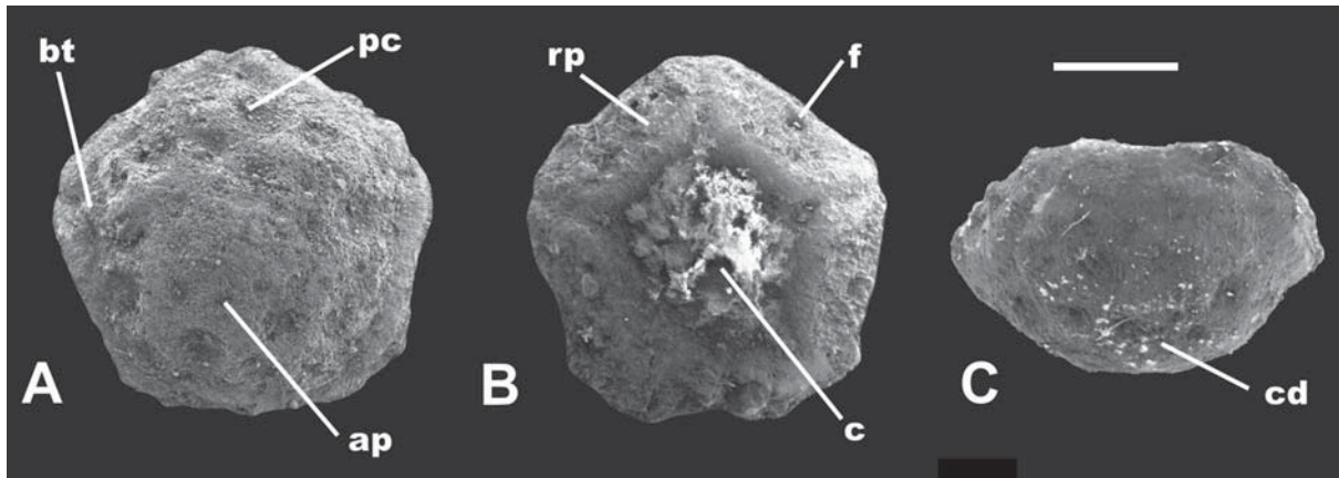
Text-fig. 5. Scanning electron microscopy of the Sievertella cf. polonica (Radwańska): calyx (PBR-01-80) from the Miocene of the Pirabas Formation. A – Dorsal view: bt – basal tubercles; pc – peripheral cirrus; ap – apical cirrus. B – Ventral view: rp – radial plate; f – fossa of radial plate; c – central cavity (infilled by rock material). C – Lateral view of calyx centrodorsal plate (cd). Scale bar = 1 mm
