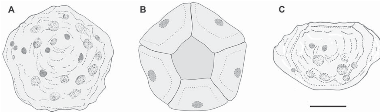
Text-fig. 6. Ink-drawing sketches of the Sievertella cf. polonica (Radwańska): calyx (PBR-01-80) from the Miocene of the Pirabas Formation. A – Dorsal view; B – Ventral view; C – Lateral view of calyx centrodorsal plate. Scale bar = 1 mm
