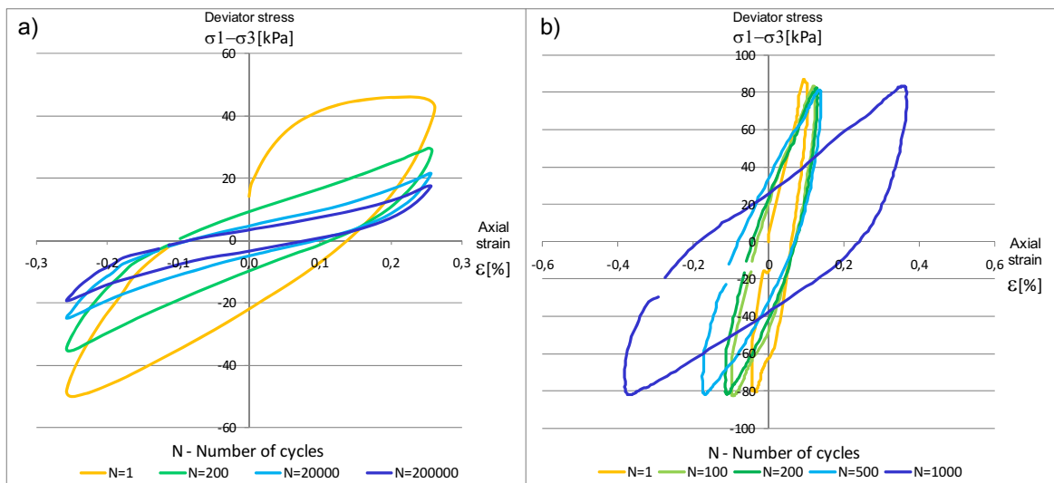
Text-fig. 9. Examples of hysteresis loops of selected load cycles with constant amplitude of (a) axial displacement (b) stress
