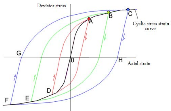
Text-fig. 10. Cyclic stress-strain curve defined as a vertex of stabilized hysteresis loop
