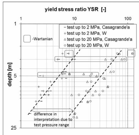
Text-fig. 20. Yield stress ratio YSR calculated for yield stresses resulted from two interpretation stress ranges and two interpretation methods
