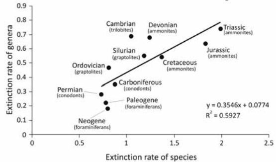
Text-fig. 4. Relationship between the average extinction rate per m. y. of the index species (curve A in Text-fig. 3) and the average proportional genus-level extinction rate (B in Text-fig. 3). Pearson’s r = 0.77 at p = 0.006 , r^2 = 0.593 ; Spearman’s r_s = 0.82 at p = 0.002 ; first differences – Pearson’s r = 0.93 at p = 0.0001 , Spearman’s r_s = 0.89 at p = 0.0005
