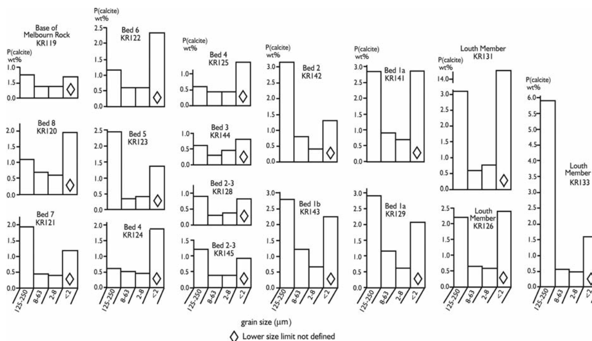
Text-fig. 11. Histograms showing the variation in phosphorus (P) within the bulk calcite of the <2 μm, 2–8 μm, 8–63 μm and 125–250 μm particle size fractions from various samples of the Plenus Marls and adjacent sediments at Shakespeare Cliff, Dover (Text-fig. 6a for sample horizons). KR131 is the only sample with a <2 μm fraction which has a phosphorus content (14 wt %) in excess of the maximum value (~2.5 wt %) recorded by Siesser (1977) for the skeletal calcite of recent and Tertiary Coccolithophoridae
