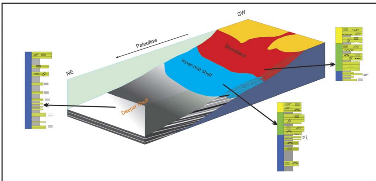
Text-fig. 10. Palaeogeographical reconstruction of Tanawal Formation representing the shoreface–deeper shelf environments. Various components such as shoreface, inner-mid and deeper shelf are indicated; for explanations see text-figure on page 4
