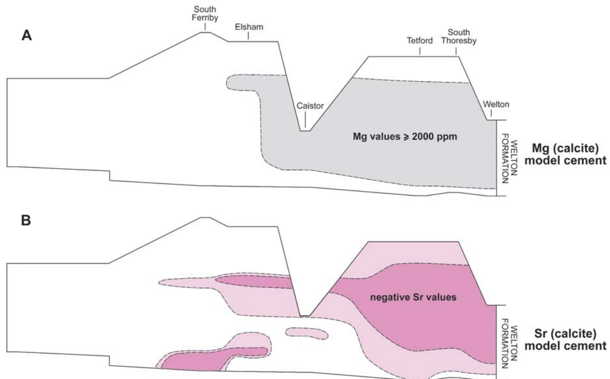
Text-fig. 19. Unit B in Lincolnshire showing the antipathetic relationship in the model cement between Mg values of 2000 ppm and above and negative values of Sr. (key as for Text-fig. 14)
