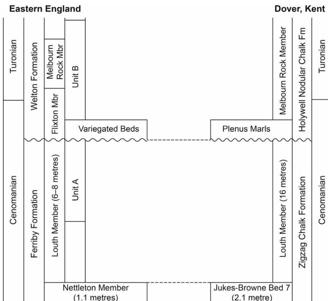
Text-fig. 4. Lithostratigraphical and stratigraphical terms used in eastern England and at Dover
