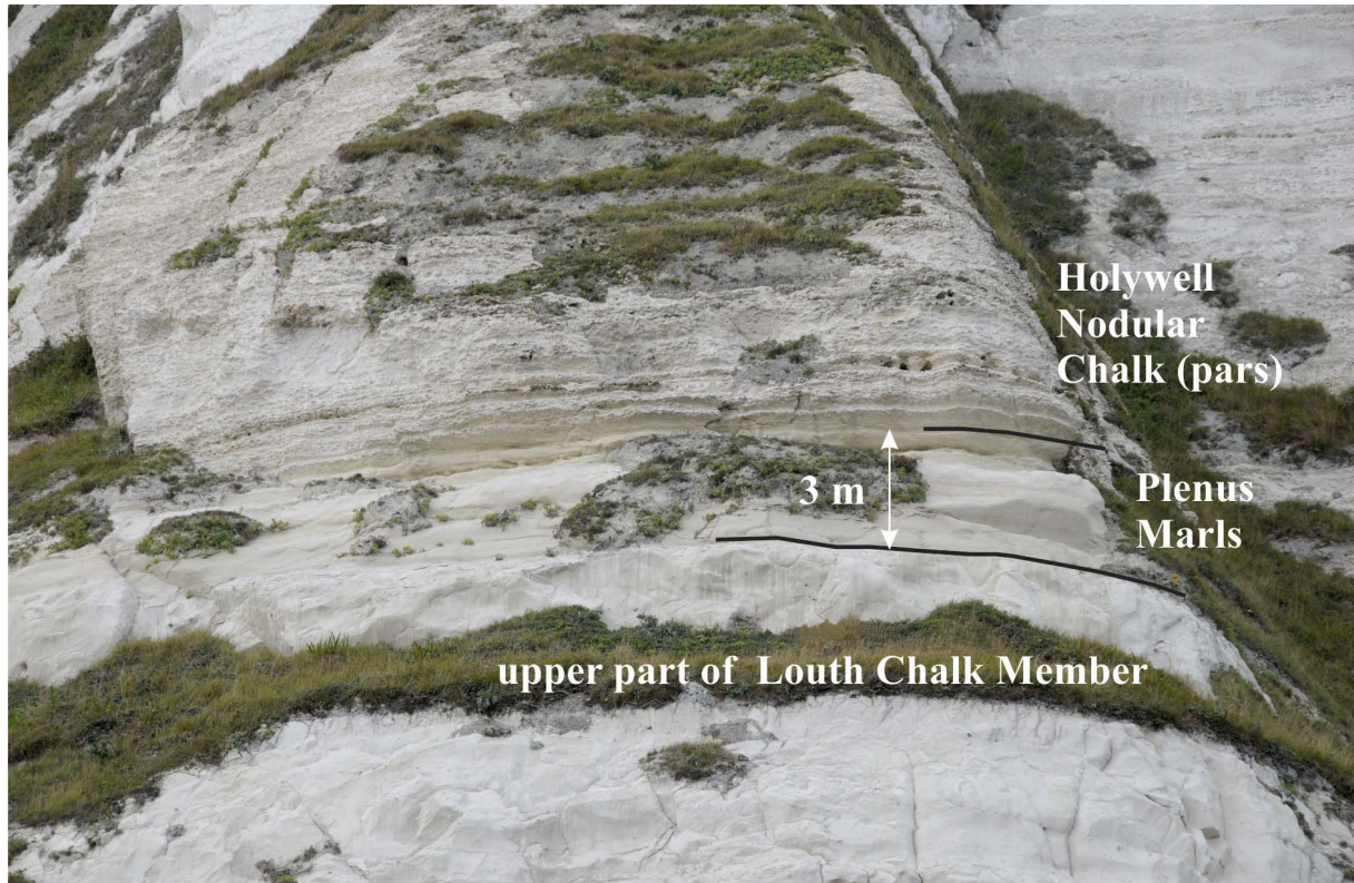
Text-fig. 6. The cliff section at Samphire Hoe, Dover, UK, showing the chalk of the upper part of the Louth Member (Zig Zag Chalk Formation), the Plenus Marls, and part of the overlying Holywell Nodular Chalk Formation
