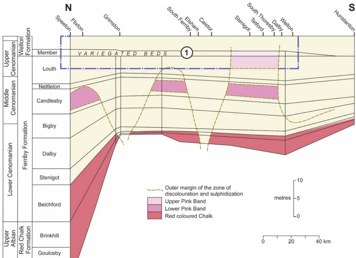
Text-fig. 3. Horizontal section of eastern England showing the overall stratigraphy of the Upper Albian, Cenomanian and Lower Turonian strata and the general distribution of red colouration including the Upper and Lower Pink Bands of Bower and Farmery (1910) and the lower band of red coloured chalk of which the Red Chalk Formation is an integral part. Zone 1 indicates the stratigraphical and regional extent of the detailed investigation of chalk hardening
