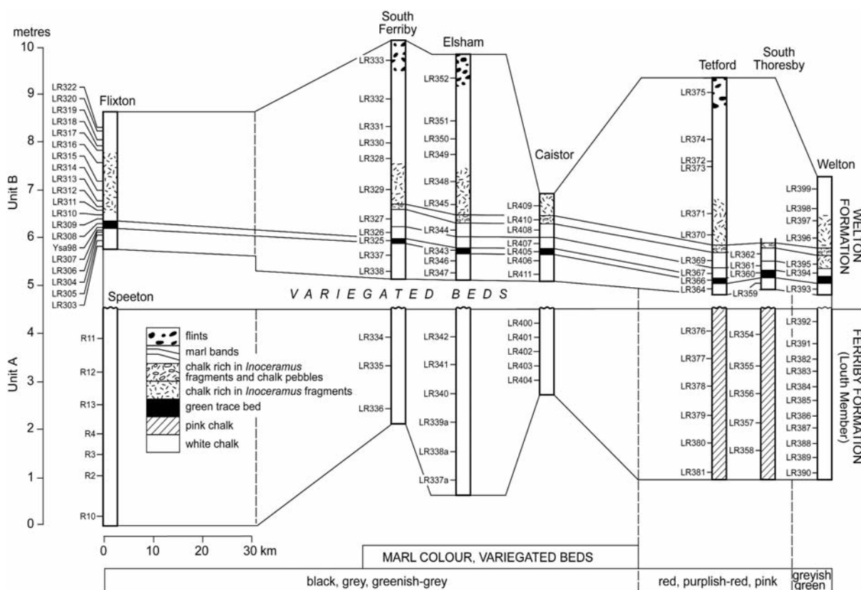
Text-fig. 5. Horizontal section through the upper part of the Ferriby Formation and the lower part of the Welton Formation in eastern England showing the position of samples in units A and B that were chemically analysed. Further details of the samples from the Louth Member at Speeton and their stratigraphic relations to other samples that have been investigated in this study as well as by Jeans et al. (2012) and Hu et al. (2014) are shown in Text-fig. 7
