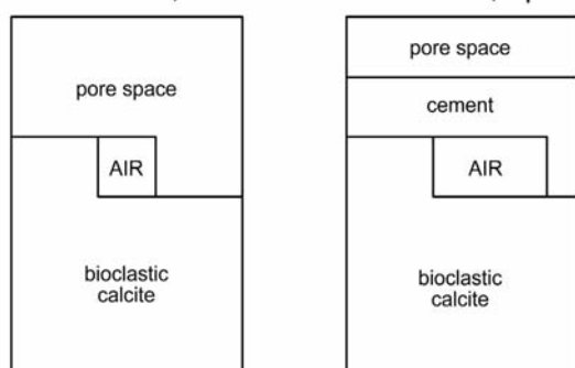
Average chalk Louth Member, Dover Sample R11 Louth Member, Speeton
