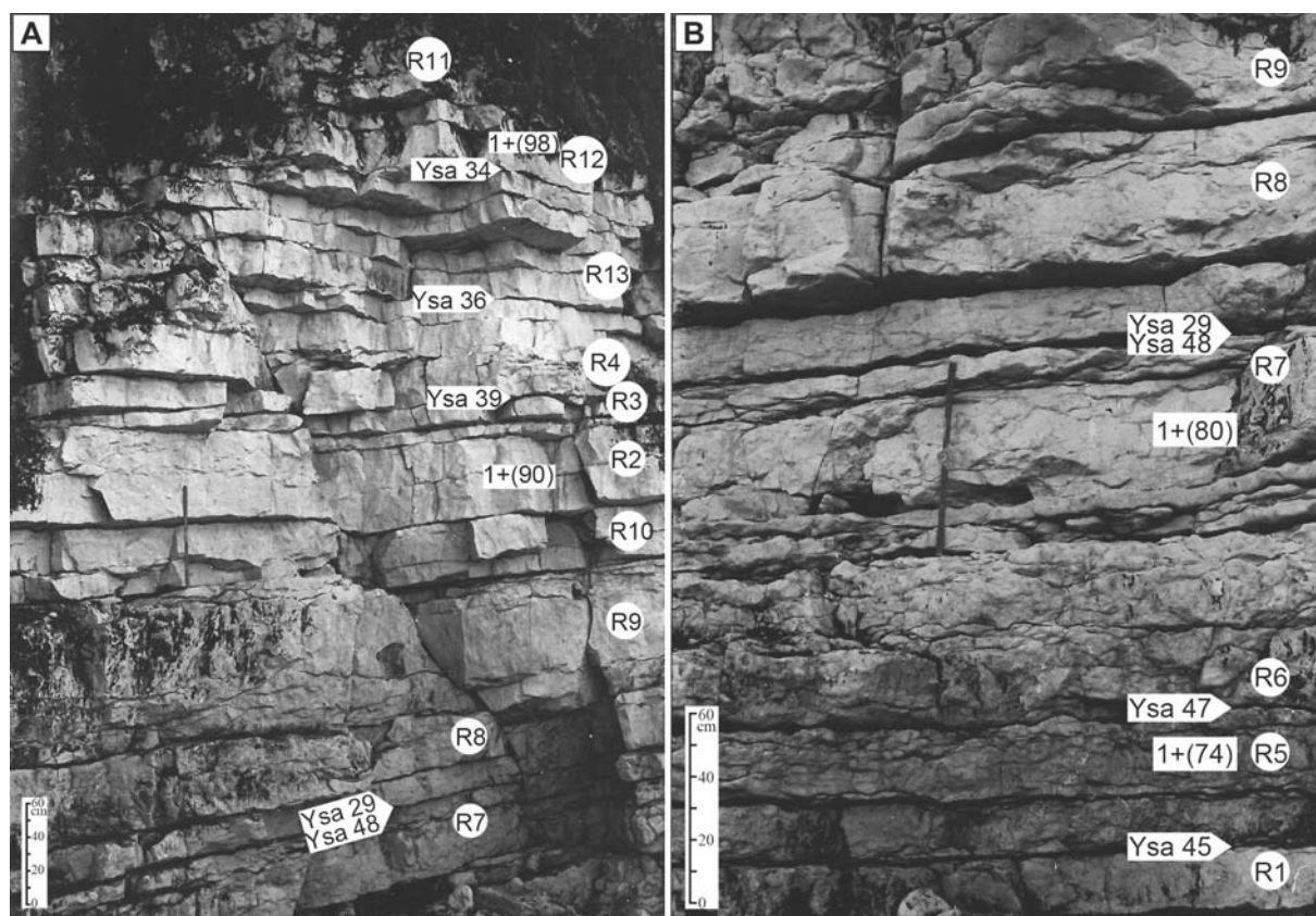
Text-fig. 7. The Louth Member of the Ferriby Formation exposed at Prentice Cove, Buckton Cliffs, Speeton, Yorkshire. This shows the position of samples investigated in this study, in Jeans et al. (2012, table 6) and in Hu et al. (2014, table 4). Text-fig. 7A shows the upper part of the Louth Member where Unit A extends down to just below sample R10 and is characterised by a laterally variable sequence of alternating beds of hard homogeneous chalk and marl seams of secondary origin. This passes gradually downwards into interbedded homogeneous and nodular chalks with intervening marl seams which are seen in Text-fig. 7B. The bed numbers (1+(98) etc.) refer to the locations of the thin sections illustrated in Text-fig. 8
