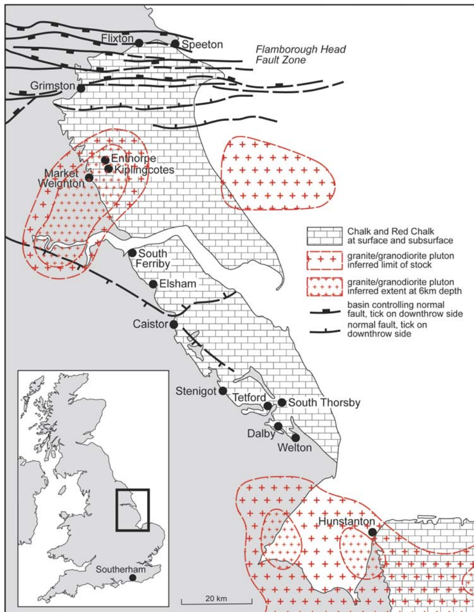
Text-fig. 21. Regional map of eastern England and the adjacent parts of the North Sea showing the distribution of the Chalk at the surface and subsurface, the main tectonic structural lines and the granites inferred to occur at depth. Based on Pharaoh et al. (1996)
