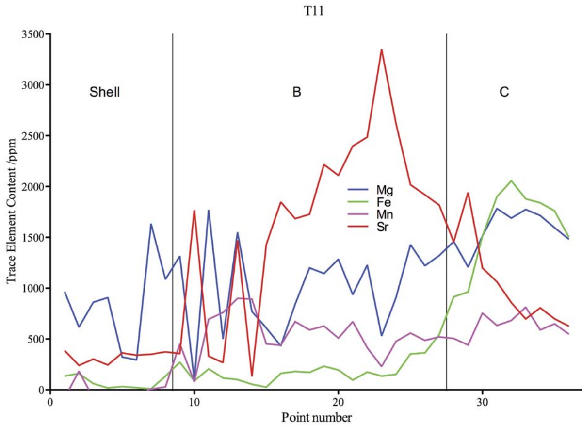
Text-fig. 18. Trace element concentrations arranged along the direction of crystal growth for zones B and C in terebratulid T11 from Unit A, Louth Member, Ferriby Formation, Speeton (Text-fig.13 of Hu et al. 2012)
