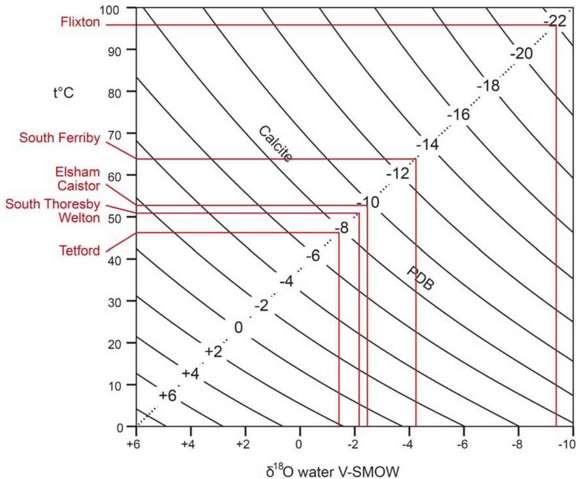
Text-fig. 20. Cross plot of temperature and \delta^{18}\text{O} for the equilibrium precipitation of calcite in sea water showing the temperatures of precipitation of the model cement in the basal chalk subunit of Unit B at various locations in eastern England
