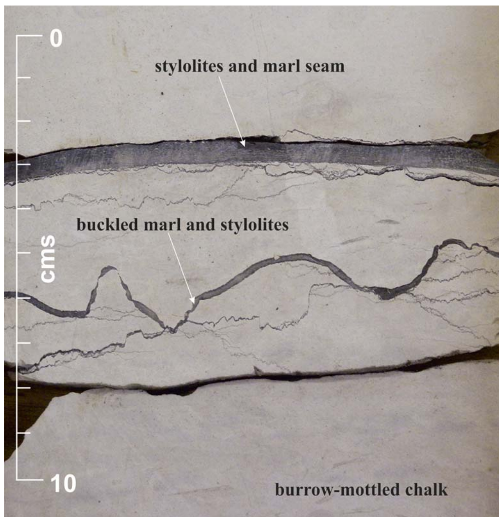
Text-fig. 25. High density white chalk (SG >1.95) from the North Sea showing primary marl seams that have been secondarily compressed and buckled in association with the development of syn-deformational stylolites and secondary marl seams. (from Mortimore, 2014, figure 5.37)
