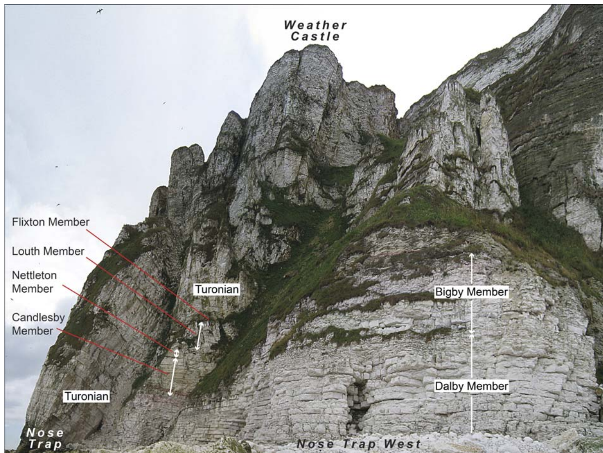
Text-fig. 1. Hard Northern Province Chalk in the Buckton Cliffs at Nose Trap, near Speeton, Yorkshire, UK. This exposes various members (Dalby, Bigby, Candlesby, Nettleton, Louth) from the middle and upper part of the Cenomanian Ferriby Formation and the Flixton Member of the overlying, Welton Formation (predominantly of Turonian age). Details of the stratigraphy and location are given, respectively, in Text-fig. 4 and in Hu et al. (2012, Text-fig. 5)
