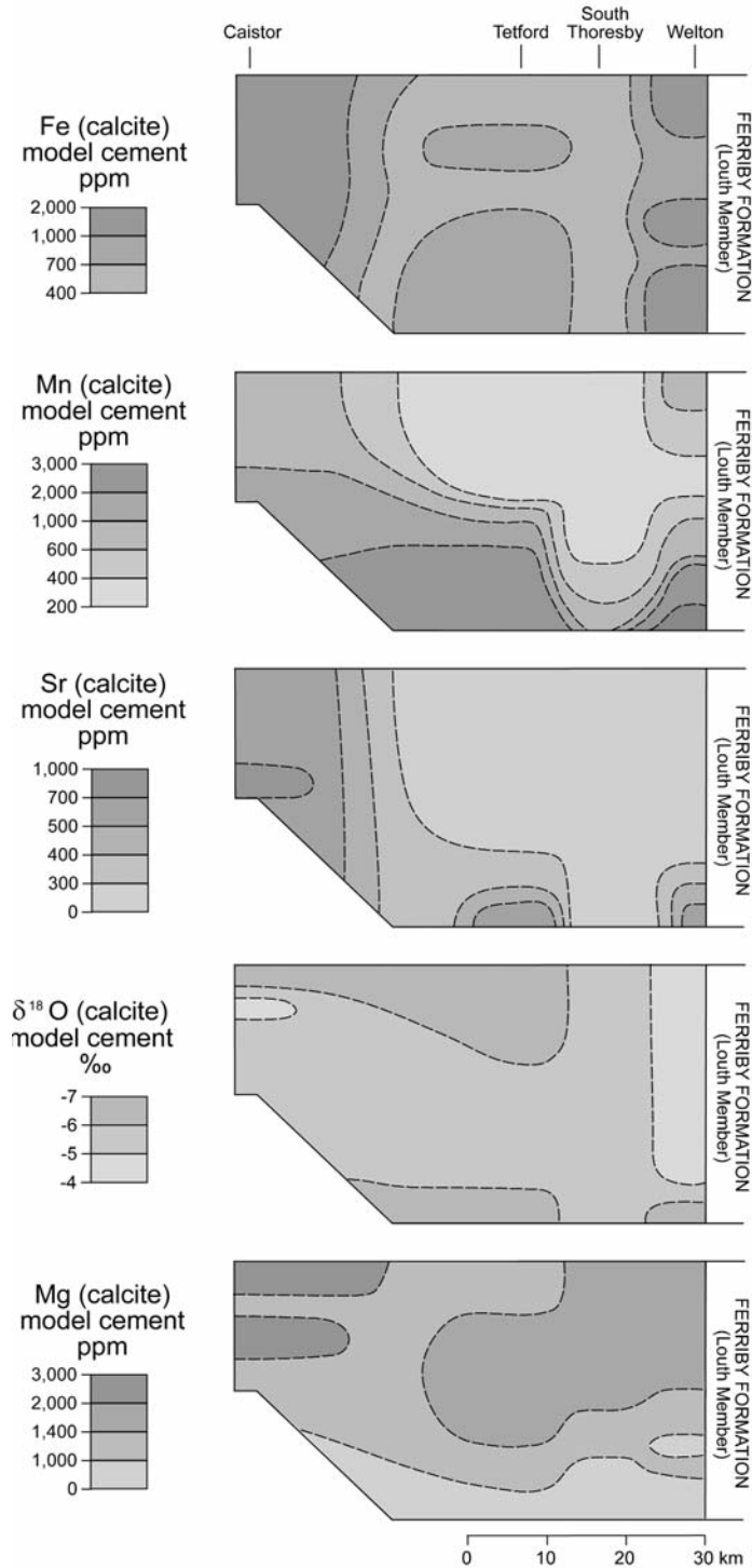
Text-fig. 17. Comparison of the variation in the model values of Fe, Mn, Mg, Sr and \delta^{18}\text{O} in Unit A between Caistor and Welton showing the general regional association of higher values of Fe and Mg with low values of Mn and Sr
