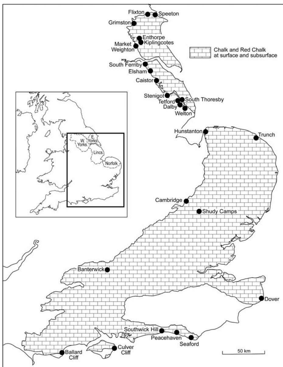
Text-fig. 2. Distribution of the Upper Cretaceous Chalk at the surface and subsurface in the UK showing the locations mentioned in the text and in Hu et al. (2014). The insert shows the county names (East Yorkshire: Lincolnshire: Norfolk) referred to in the text
