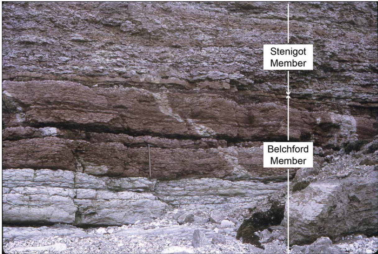
Text-fig. 22. The Ferriby Formation at Red Cliff, Speeton showing the Belchford Member overlain by the Stenigot Member. The lower part of the Belchford is bluish-greyish white as a result of sulphidization and contains pyrite and marcasite crystals. Three narrow zones of sulphidization extend upwards on either side of inclined fractures that cross-cut the reddish brown coloured chalk of the upper part of the Belchford Member. These disappear into the marbled pink and white nodular chalk of the overlying Stenigot Member. Scale, ice axe, 86 cm
