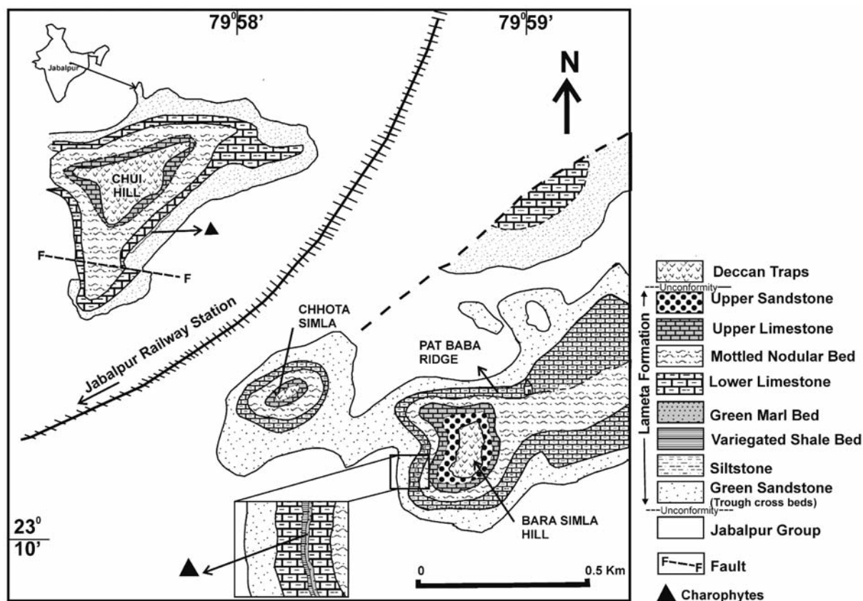
Text-fig. 1. Geological map of the Jabalpur Cantonment area, Madhya Pradesh, showing the charophyte-bearing levels (map modified after Matley 1921). Enlarged views of the inset map (not to scale) showing the presence of the variegated shale and the charophyte-bearing green marl bed, which are intercalated within the Lower Limestone
