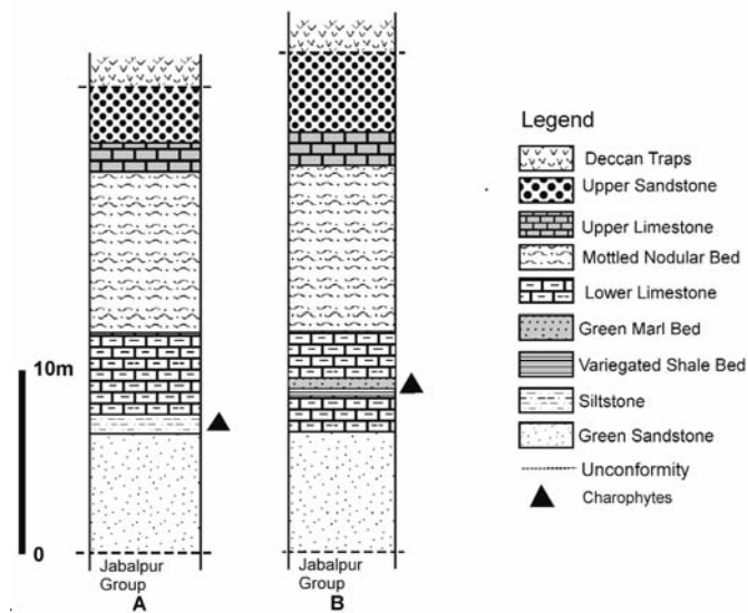
Text-fig. 2. Stratigraphic successions of the Lameta Formation at Chui Hill (A) and Bara Simla Hill (B), showing the charophyte-bearing levels
