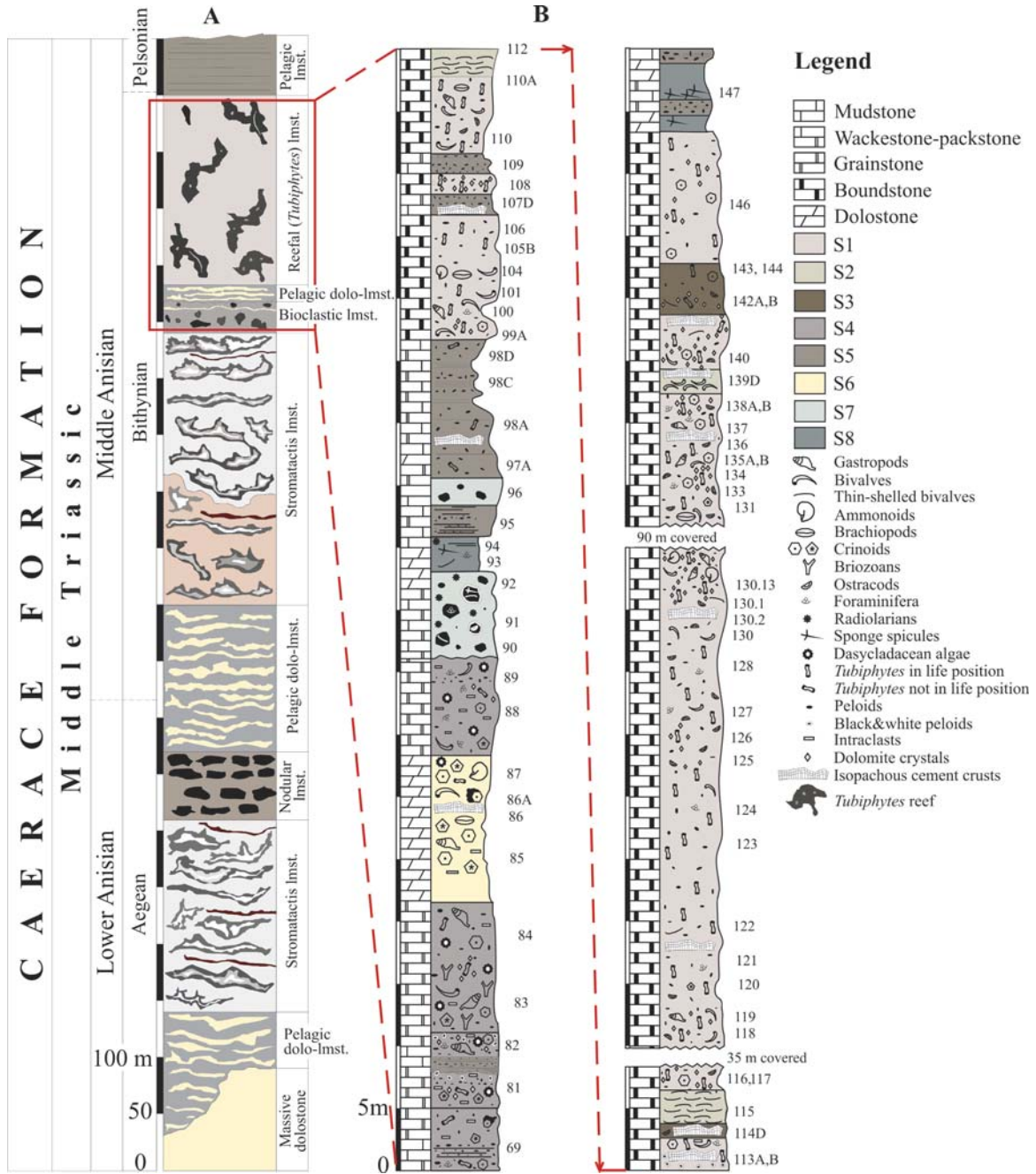
Text-fig. 4. Synthetic lithological column (A) of the Middle Anisian Caerace Formation in the Mahmudia Quarry, and detailed lithofacies column (B continued) of the studied section (marked by the red quadrangle) with sample log for the lower Middle Anisian (Bithynian) Tubiphytes -buildup. Symbols S1 to S8 as shown in Text-fig. 3 and Table 1
