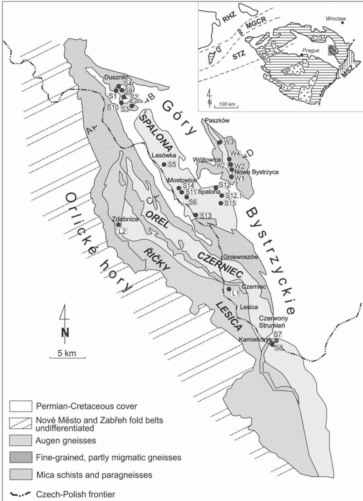
Text-fig. 1. Geological sketch of the western limb of the Orlica-Snieżnik Dome, with location of sampling sites. Modified after Dumicz (1964), Opletal et al. (1980) and Don et al. (2003). Inset: Map location (shaded box) within the wider context of the Bohemian Massif (horizontal rulings). Abbreviations are as follows: MGCR (Mid-German Crystalline Rise); MSZ (Moravo-Silesian Zone, vertical ruling); RHZ (Rhenohercynian Zone); STZ (Saxothuringian Zone, horizontal dashed ruling); Variscan granitoids (crosses)
