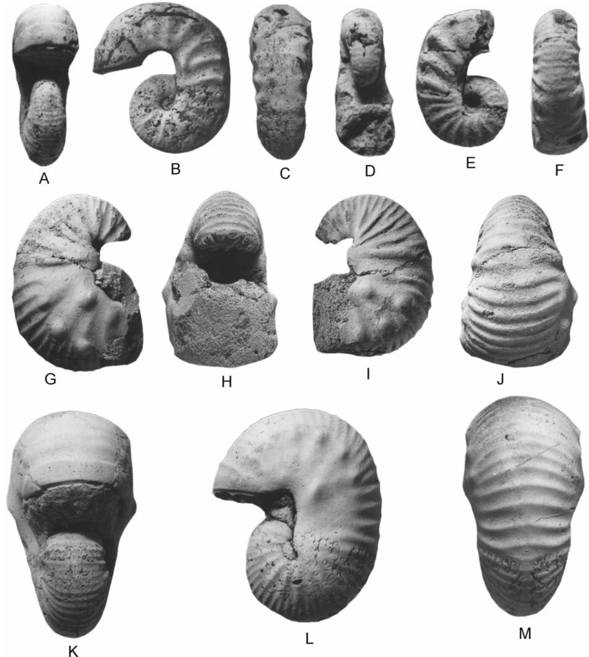
Text-fig. 1 A-M – Scaphites reeseidei Collignon, 1969. A-C – the holotype of Scaphites aquisgranensisiformis Collignon, 1969, p. 53, pl. 533, fig. 2100, from the Lower Campanian Scaphites reeseidei Subzone of the Karapadites karapadensis Zone, gisement 170 of Collignon's Berere I (Belo sur Tsiribihina) section, Madagascar. D-F – SAM4826, the original of Scaphites sp. of Woods, 1906, p. 343, pl. 44, fig. 8, from the Santonian to Lower Campanian Mzamba Formation at locality 1 of Kennedy and Klinger (1975). G-J – SAM-PCZ22273, from the same horizon and locality as D-F. K-M – the holotype of Scaphites reeseidei Collignon, 1969 p. 51, pl. 533, fig. 2098, from the Lower Campanian Scaphites reeseidei Subzone of the Karapadites karapadensis Zone, gisement 712 of Collignon's Ampamba-Antsirasia (Belo sur Tsiribihina) section, Madagascar. All figures are \times 1.5 .
