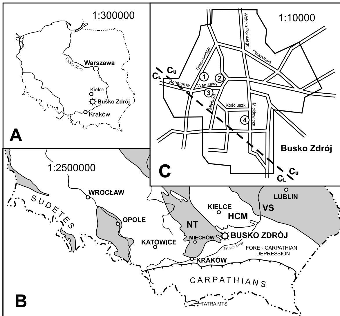
Fig. 1. Location and regional geology of the Busko Zdrój area. A – Map of Poland. B – Simplified geological map of southern Poland; areas of Cretaceous deposits exposed at the surface or under a Quaternary and continental Paleogene or Neogene cover are gray-coloured; NT – Nida Trough, HCM – Holy Cross Mountains (Palaeozoic core plus Triassic and Jurassic margins); VS – Vistula sections (modified from MARCINOWSKI & RADWAŃSKI 1983, fig. 1). C – Location of ammonite-bearing outcrops (1-4) in Busko Zdrój; C_L – Lower Campanian, C_U – Upper Campanian (based on the Geological Map of Poland, file Busko Zdrój)
