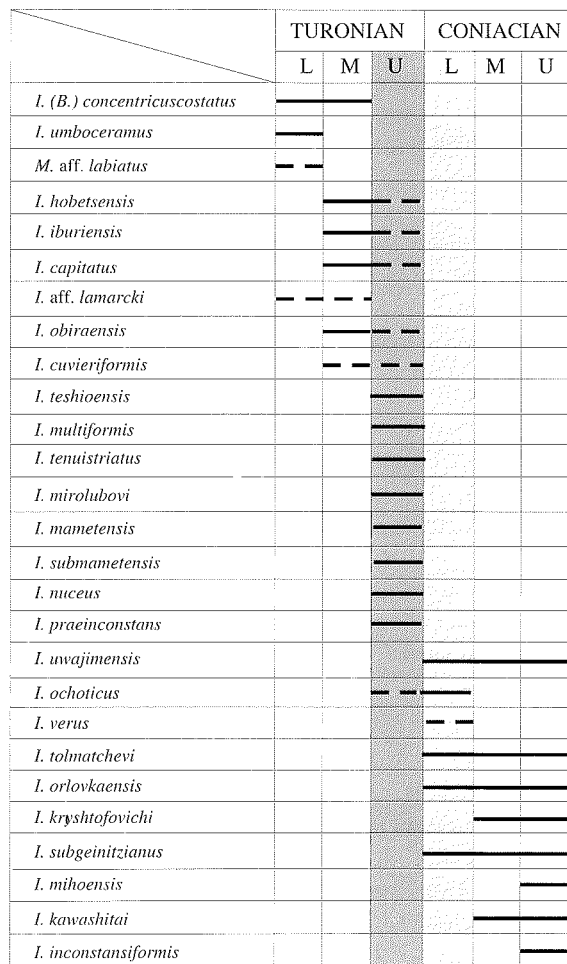
Fig. 4. Stratigraphic distribution of the Turonian – Coniacian inoceramids in the Russian Pacific coast succession
